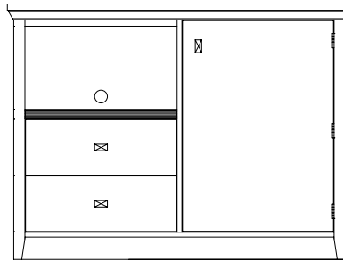
Minibar Chest 2719A23A15 W 53 7/8 D 23 3/4 H 40 (W 1370mm D 605mm H 1015mm) Minibar cavity dim 23 3/16w x 20 1/8d x 33 1/4h (590mm x 510mm x 845mm) Microwave cavity dim 23 13/16w x 20 7/8d x 13h (605mm x 530mm x 330mm)
