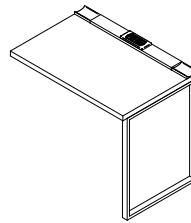
Desk 3639A25BNR-B 36 x 23 7/8 x 31 3/64
