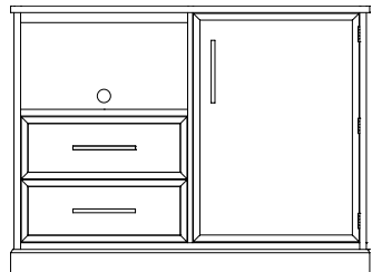
Minibar Chest 2710A23A15 W 53 7/8 D 23 3/4 H 40 (W 1370mm D 605mm H 1015mm) Minibar cavity dim 24 7/16w x 20 3/8d x 34 1/2h (620mm x 520mm x 875mm) Microwave cavity dim 25 1/16w x 21 3/8d x 13h (635mm x 545mm x 330mm)
