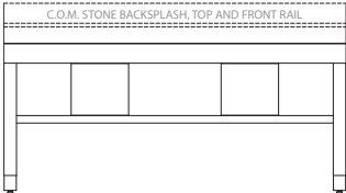
Double Vanity (K/D) (COM stone/sink) 2867A21C15 G-101-18 68 1/2 x 22 x 33 1/4
