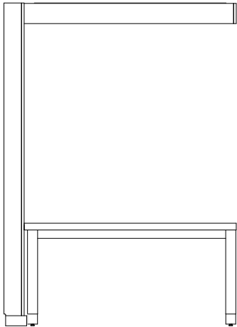
Dining Table G-102-01 2867A07A15 1 of 3 Top Ceiling Panels G-101-26 2867A25H15-A 2 of 3 Wall Panels & Scribe Rails G-101-26 2867A25H15-B 3 of 3 63 x 39 x 94 3/4
