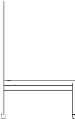
Desk (K/D) (left shown) 2867A05A15L/R 1 of 3 Top Ceiling Panels 2867A25B15-A 2 of 3 Wall Panels & Scribe Rails 2867A25B15-B 3 of 3 G-101-11L/R 57 1/2 x 22 x 94 3/4
